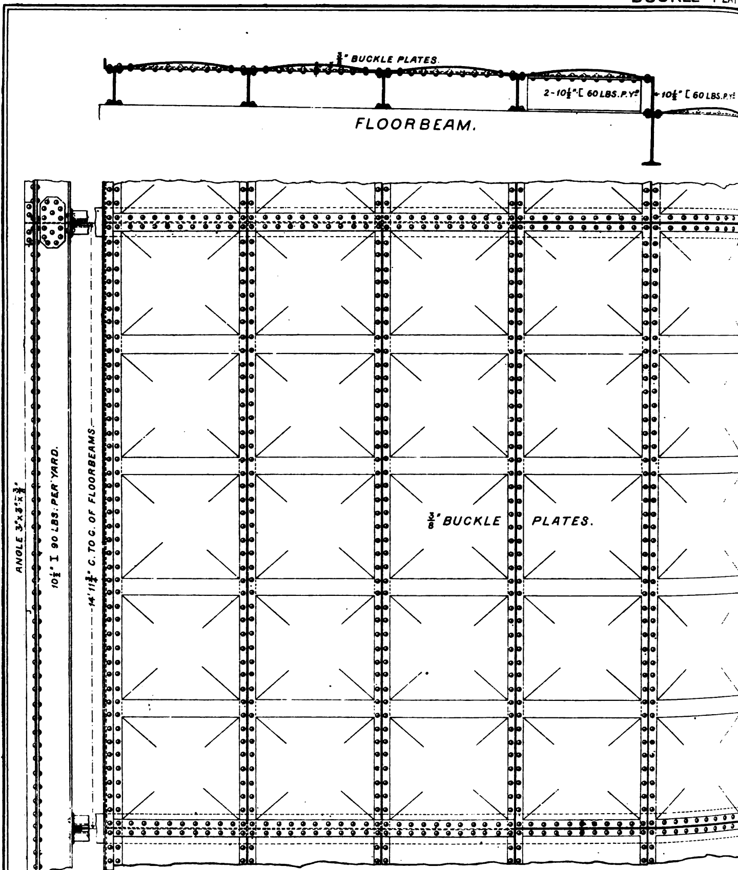
GENERAL PLAN OF BUCKLE PLATES.
