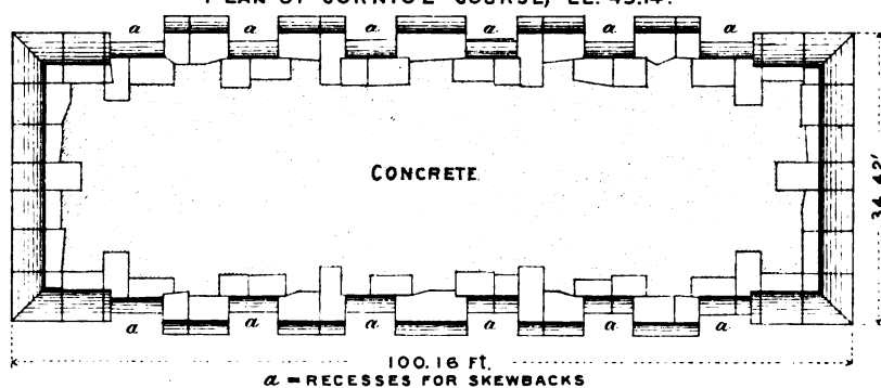
PLAN OF CORNICE COURSE, EL. 45.14.
