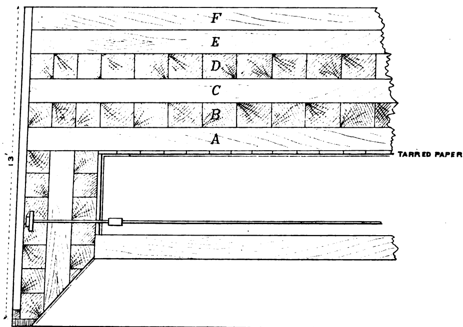
ENLARGED END OF CROSS SECTION.
