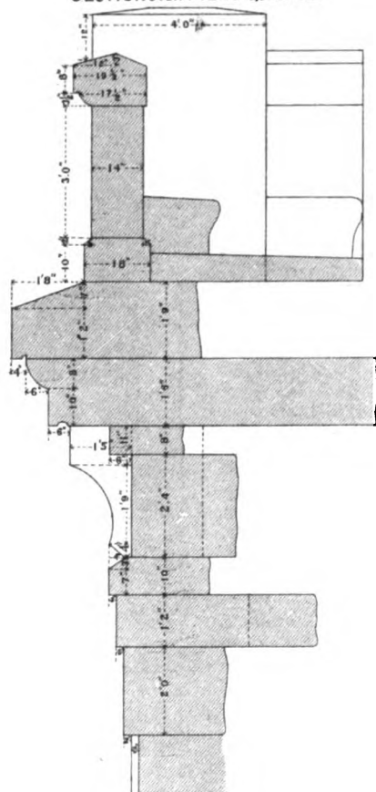
SECTION OVER PIERS I, II AND III.
