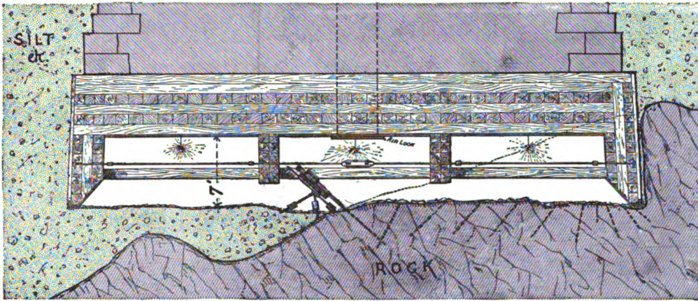
CAISSON FOUNDATION, CENTRAL PIER, WASHINGTON BRIDGE, NEW YORK CITY.
