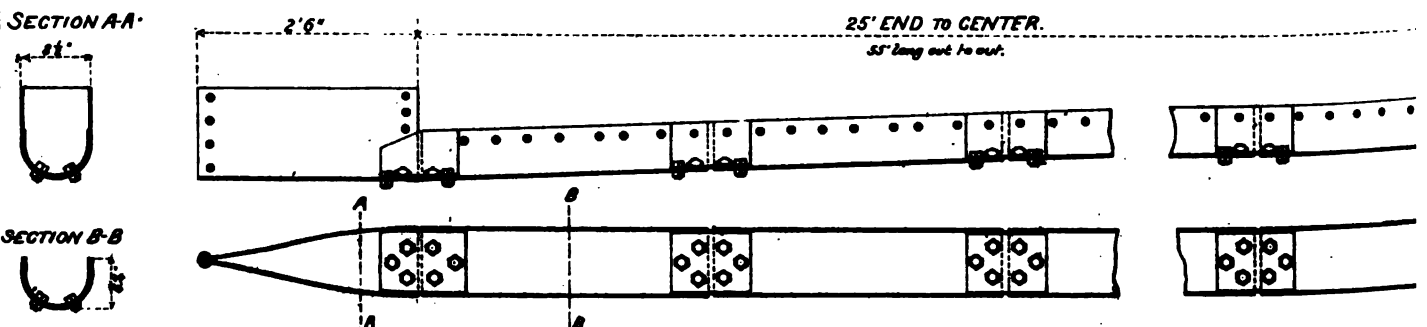
EXPANSION TROUGH
