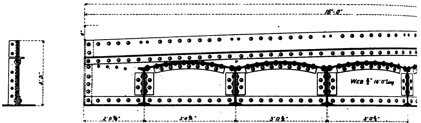
ELEVATION of SLIDING BEAM. END of IRON FLOORING.
