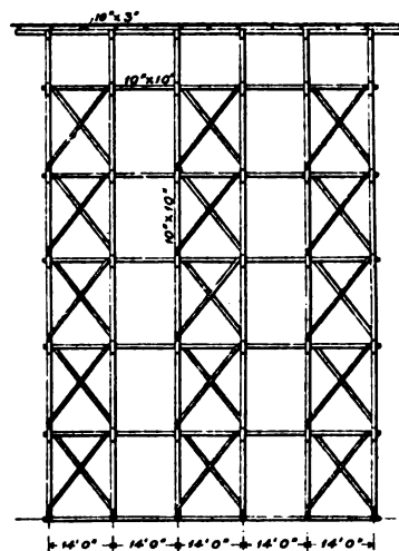
CROSS SECTION.
