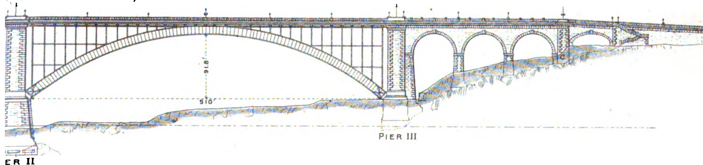
BRIDGE AS BUILT, (WASHINGTON BRIDGE)
