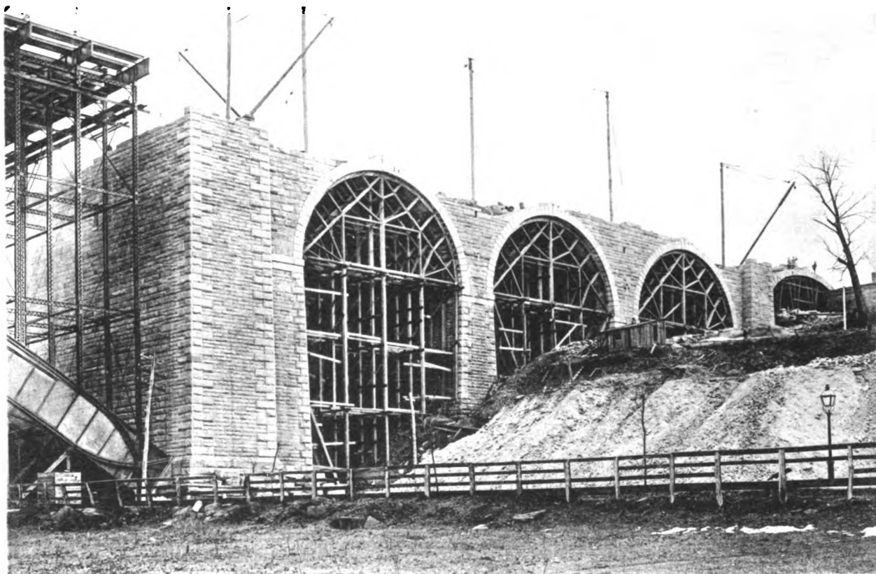
RIVER AND LAND SPANS, MARCH 23, 1888.
