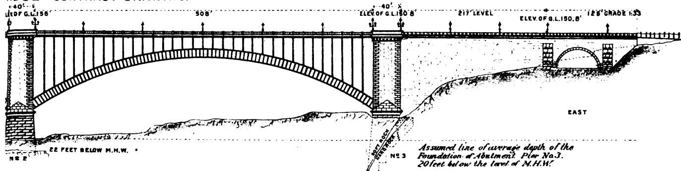
BRIDGE - CONTRACT DRAWING.
