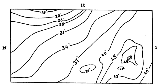
CONTOURS OF ROCK SURFACE UNDER CAISSON ELEVATIONS BELOW DATUM.
