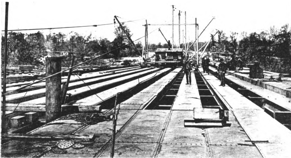
RIVER SPAN, MAY 18, 1888. SHOWING BUCKLE PLATES.
