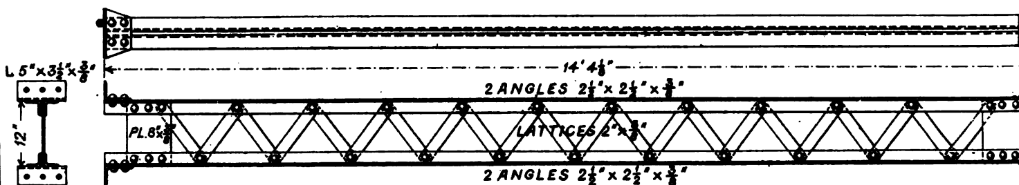
LONGITUDINAL INTERMEDIATE STRUTS.
