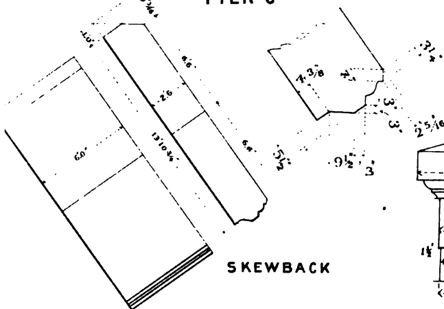
PIER C
