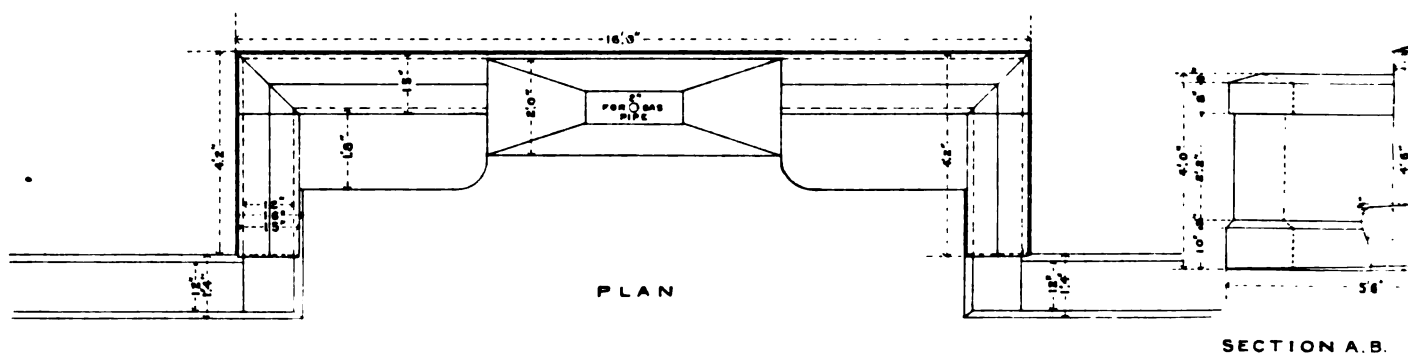
SECTION OVER PIERS I, II AND III.
