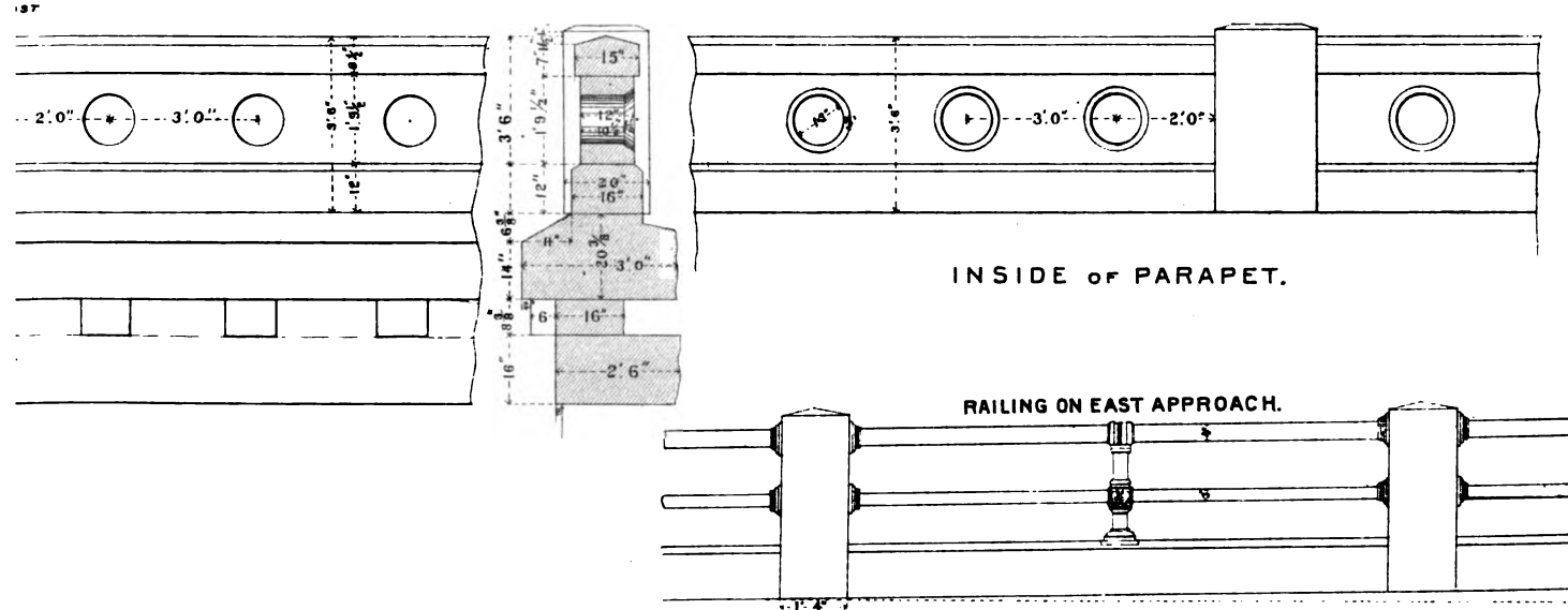
PARAPET OVER APPROACH.
