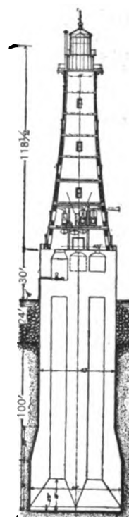
Diamond Shoal Light House, now under construction.
