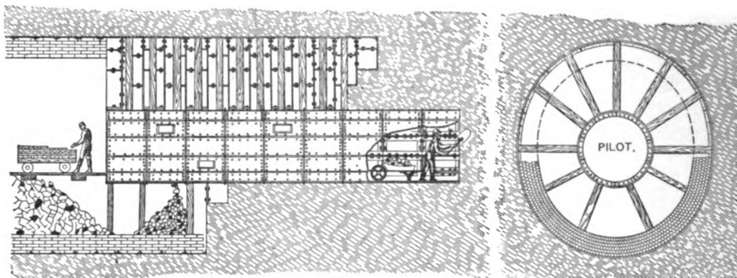
ANDERSON'S SYSTEM OF TUNNELING.
