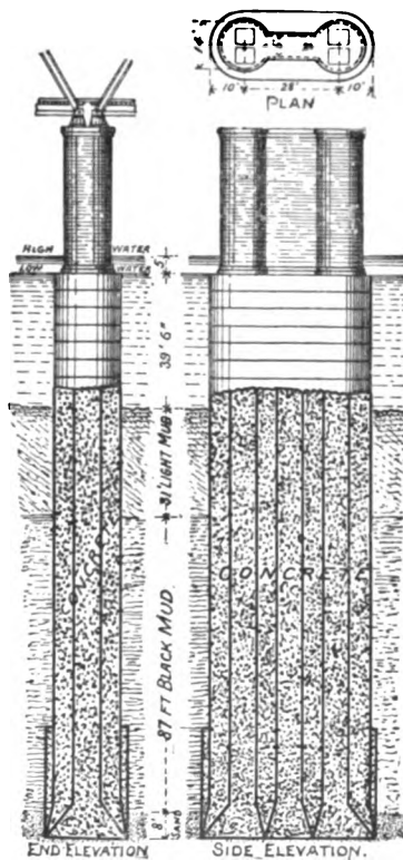
Pier Foundations of the Hawksbury Bridge, N. S. W., Australia.
