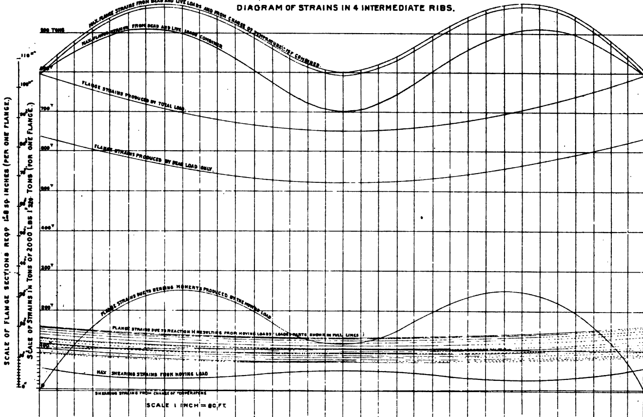
DIAGRAM OF STRAINS IN 4 INTERMEDIATE RIBS.
